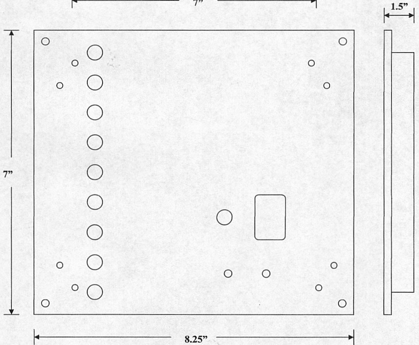
SWITCHING UNIT P/N GP5009
